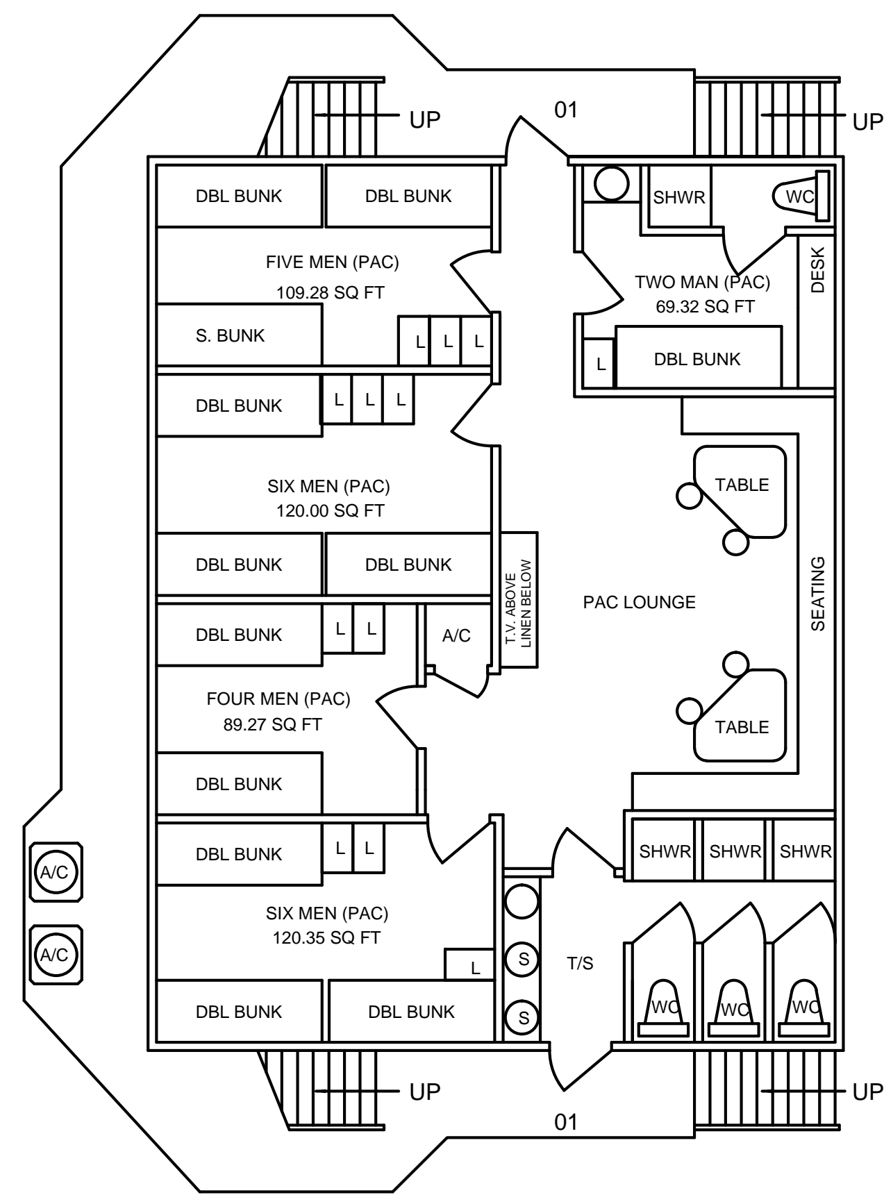
DMI CLASS 175 LIFTBOAT GENERAL ARRANGEMENT - LEVEL 01 (22 BERTHS)
