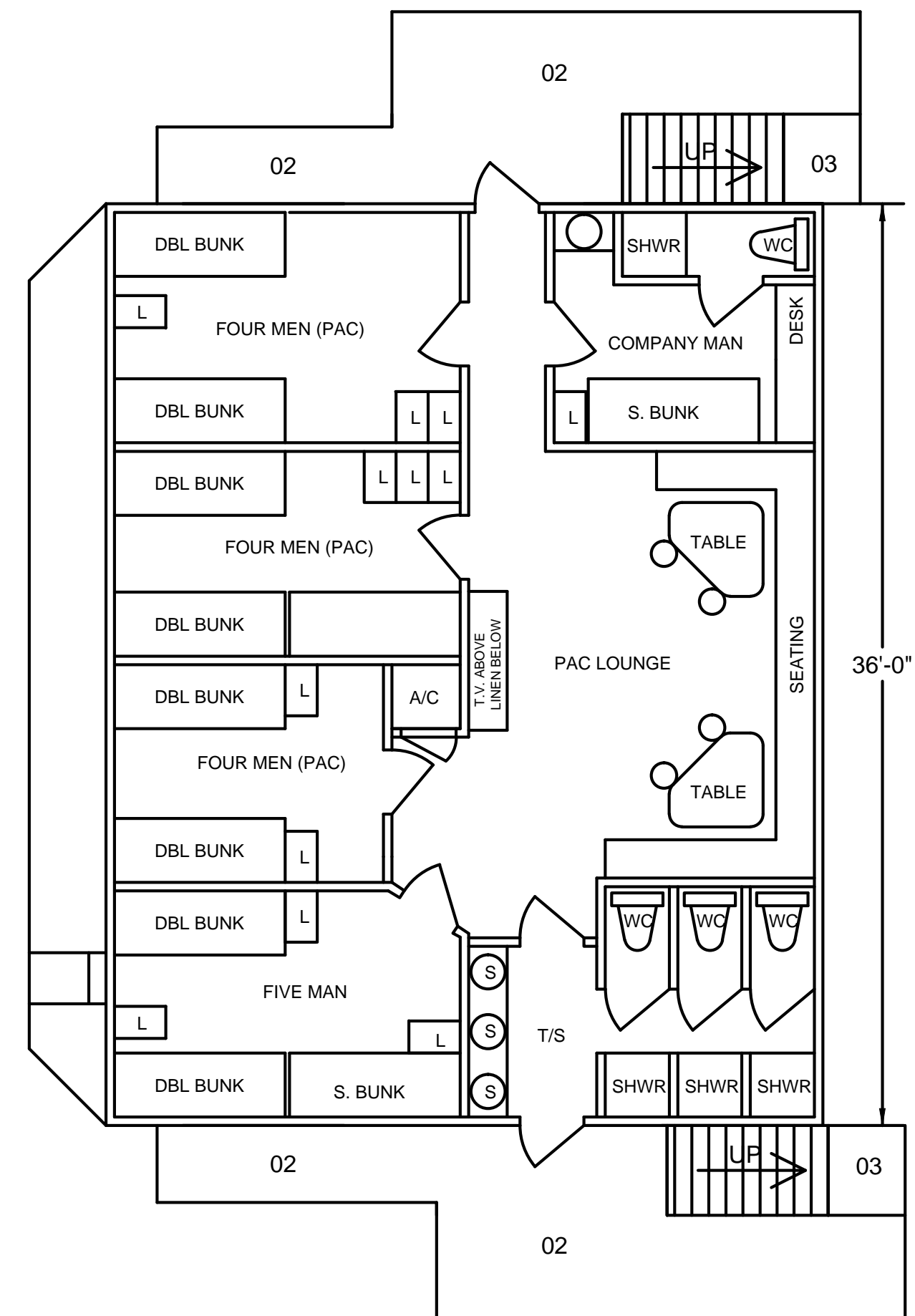
DMI CLASS 200 LIFTBOAT GENERAL ARRANGEMENT - LEVEL 02
