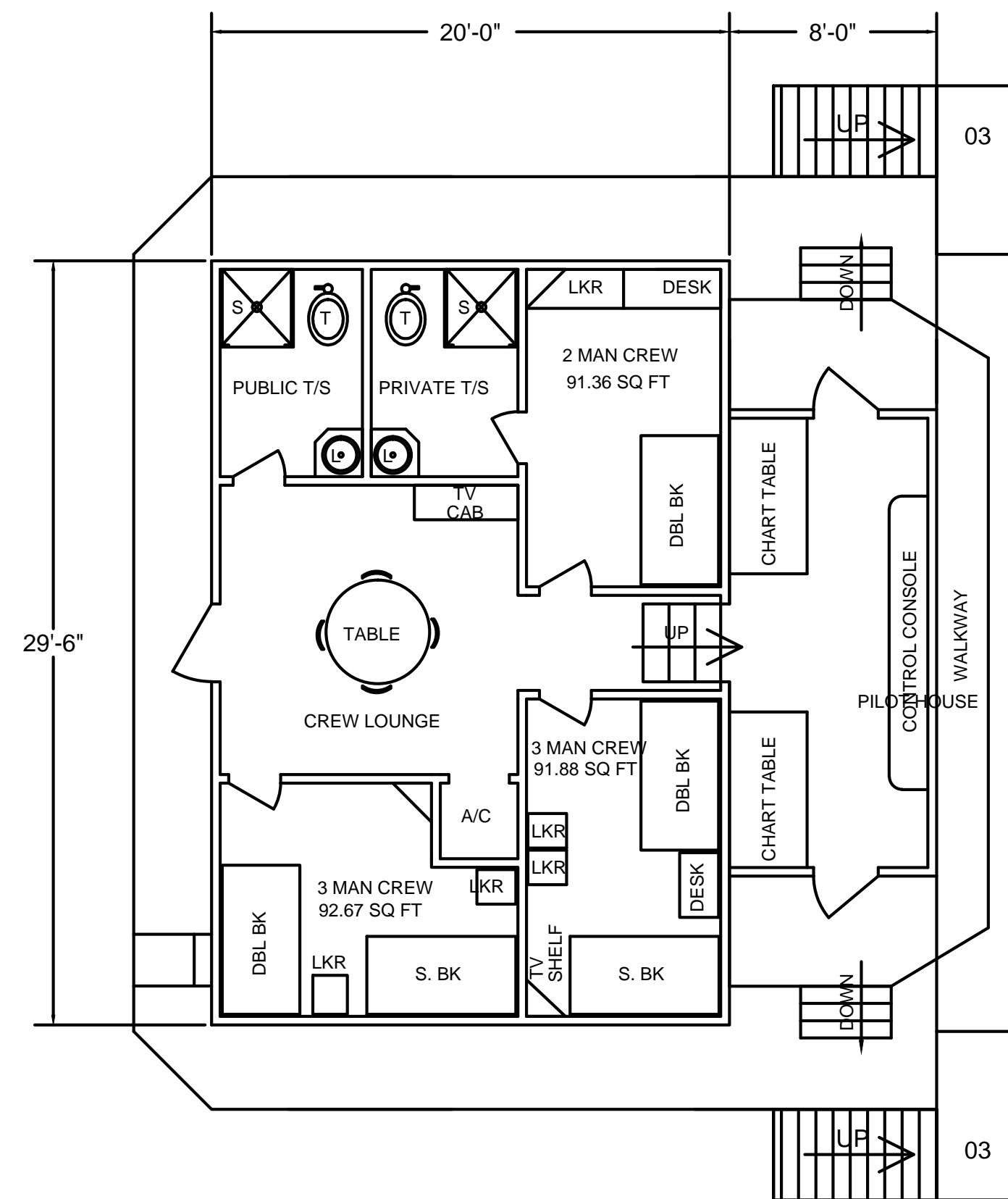
DMI CLASS 215 LIFTBOAT GENERAL ARRANGEMENT - LEVEL 03
